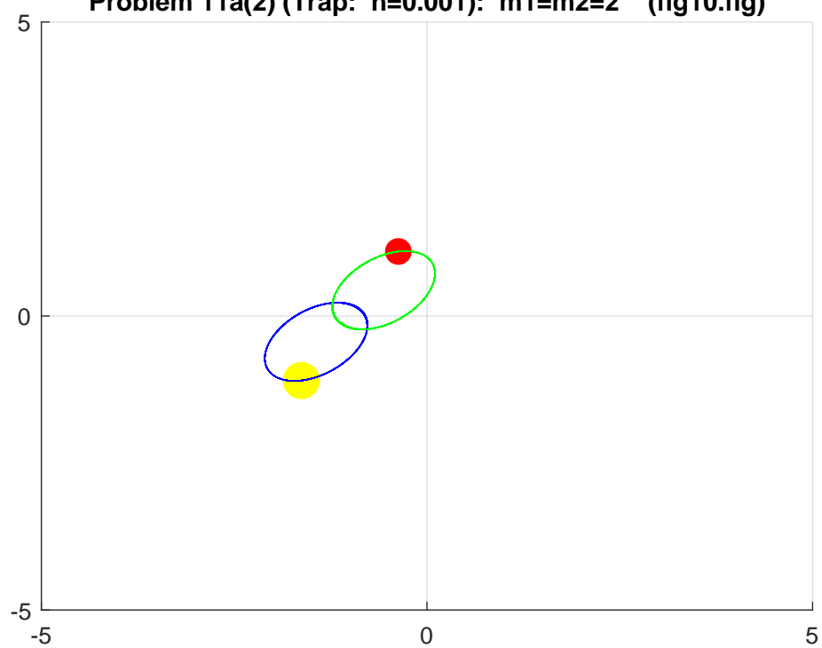
Celestial Mechanics: Two (2) Body Problem Problem 11a(2) (Trap: h=0.001 ): m_1=m_2=2 (fig10.fig)
